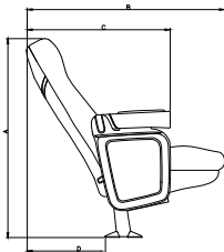
A Back height B Seat in down position C Rise of back to front of armrest D Back pitch allowance E Chair width Back height 20" 21" 23" 24" 39" 39" 39" 39"
