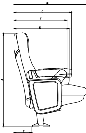
A Back height B Seat in down position C Seat in up position D Rise of back to front of cupholder armrest E Back pitch allowance F Rise of back to front of regular armrest Seat width fixed or lounge 21" 22" 23" 24" Seat width rocker 22" 23" 24" 25" Back Height 42"
